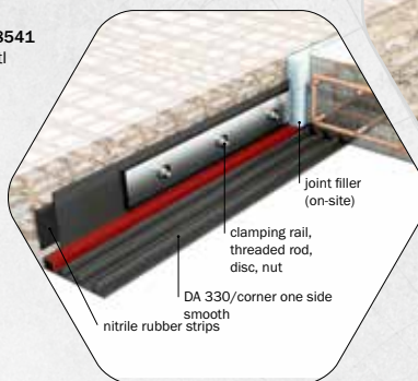
KRASOflex® Clamp Construction - external
